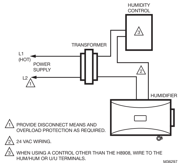
Wiring with another humidistat/thermostat.
