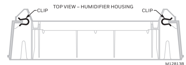
Fig. 4. Position securing clips.
