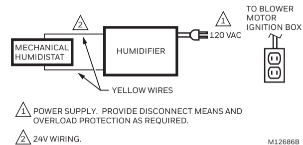
Fig. 8. Typical wiring diagram for humidifier using fan control to cycle blower motor fan and humidifier simultaneously.
