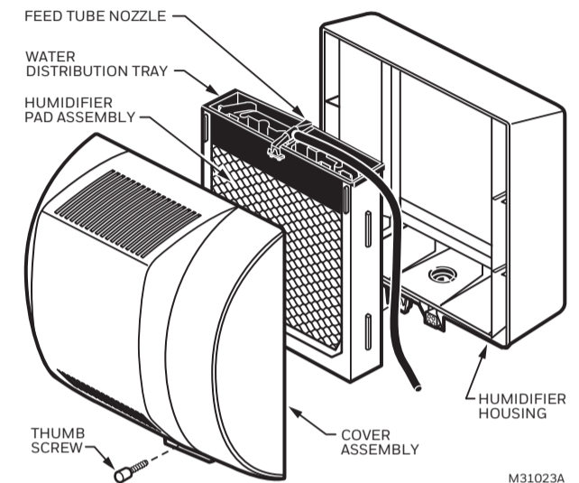
Fig. 3. Humidifier components.
