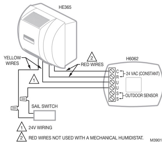
Fig. 5. Typical wiring diagram of sail switch with humidifier.
