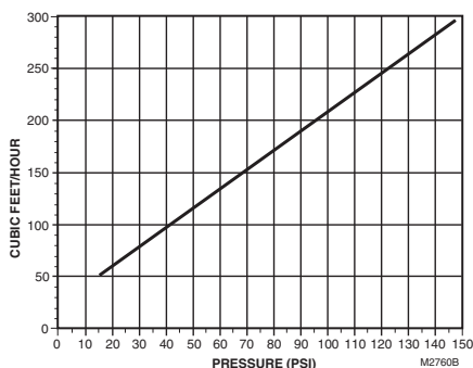
Fig. 2. EA79 flow capacities, with leakage guard cap.
