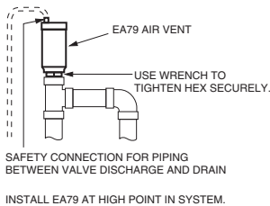
Fig. 3. Install the EA79 at high point in system.
