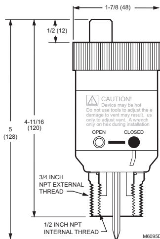
Fig. 1. EA79 dimensions in in. [mm].
