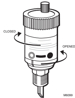
Fig. 4. Turn vent body counterclockwise to open or clockwise to close.
