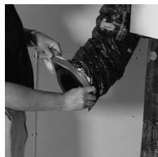
Finish by taping the vapor barrier to the collar to ensure proper seal.
