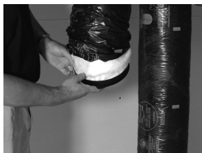
Insert insulation inside the double collar.
