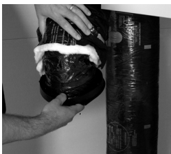
Insert vinyl duct over the hooks and seal with a Tie wrap
