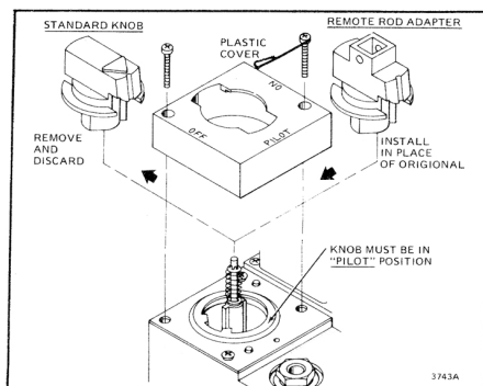
Fig. 1. Installation of 390795 Remote Rod Adapter.
