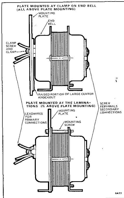
Fig. 2—Plate may be mounted to transformer in one of two positions.
