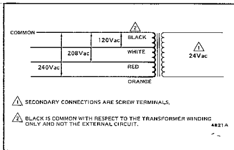
Fig. 7—Transformer schematic.
