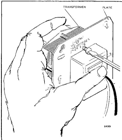
Fig. 5—Secure plate to transformer with mounting screw.
