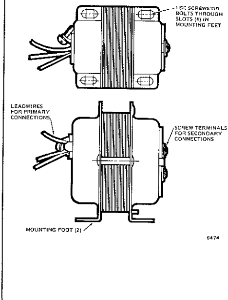
Fig. 1—Foot mounting.
