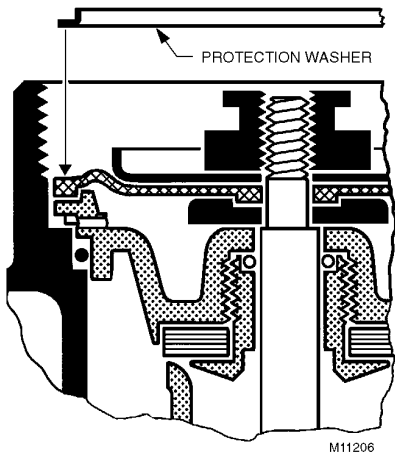
Fig. 6. Replacing Protection Washer.
