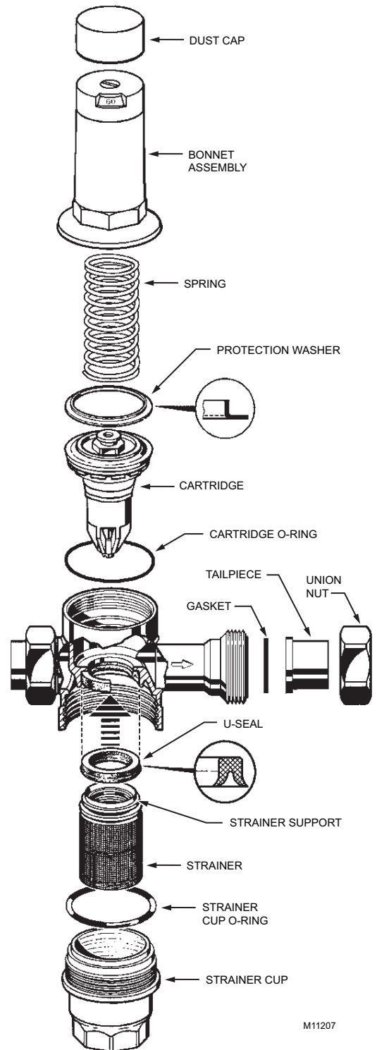
Fig. 7. Internal Parts.
