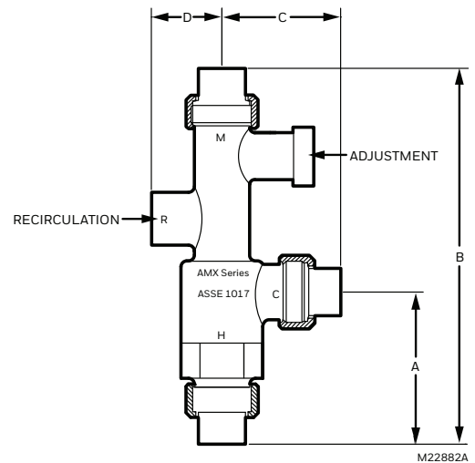
Fig. 8. Thermostatic Mixing or Diverting Valve Dimensions.
