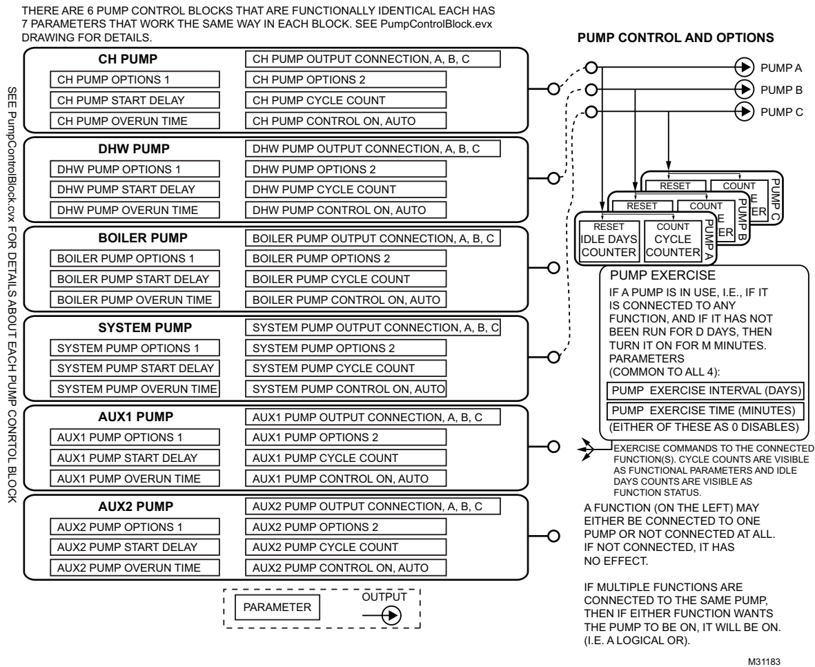
Fig. 21. Pump control blocks.
