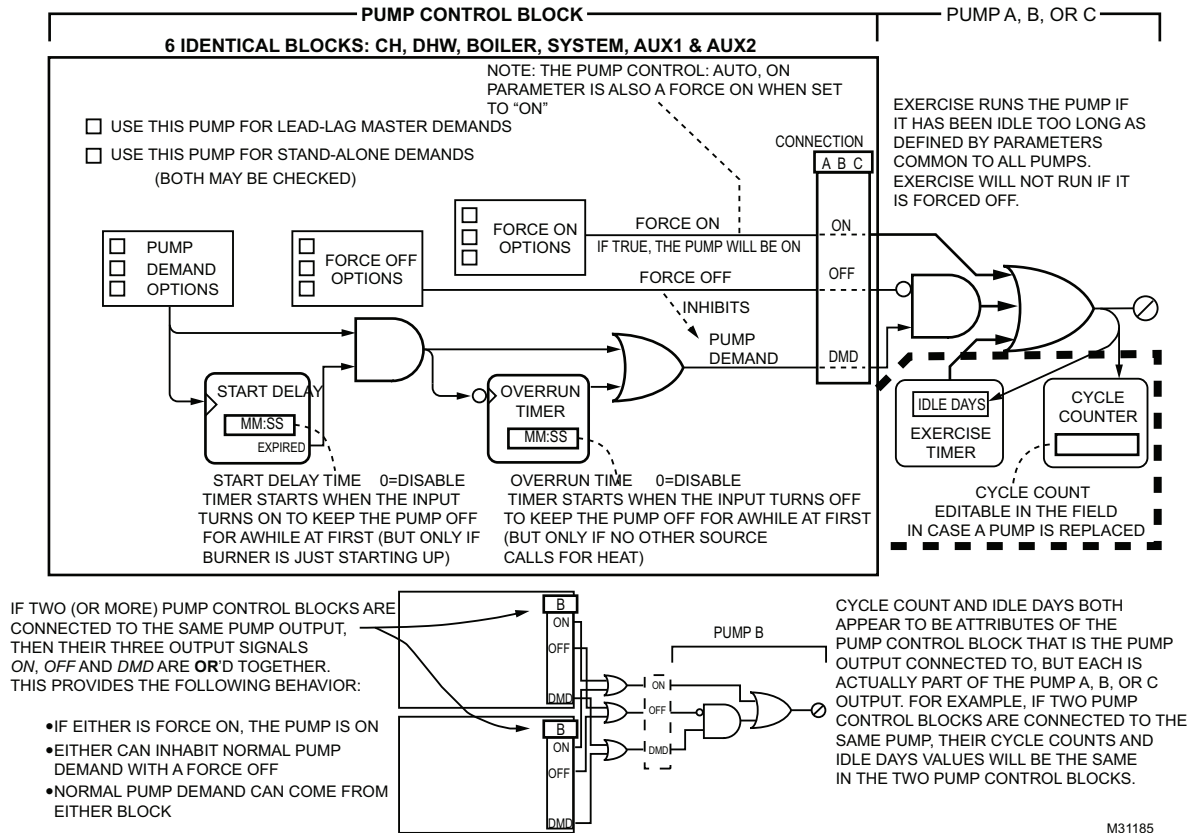
Fig. 22. Pump control block.
