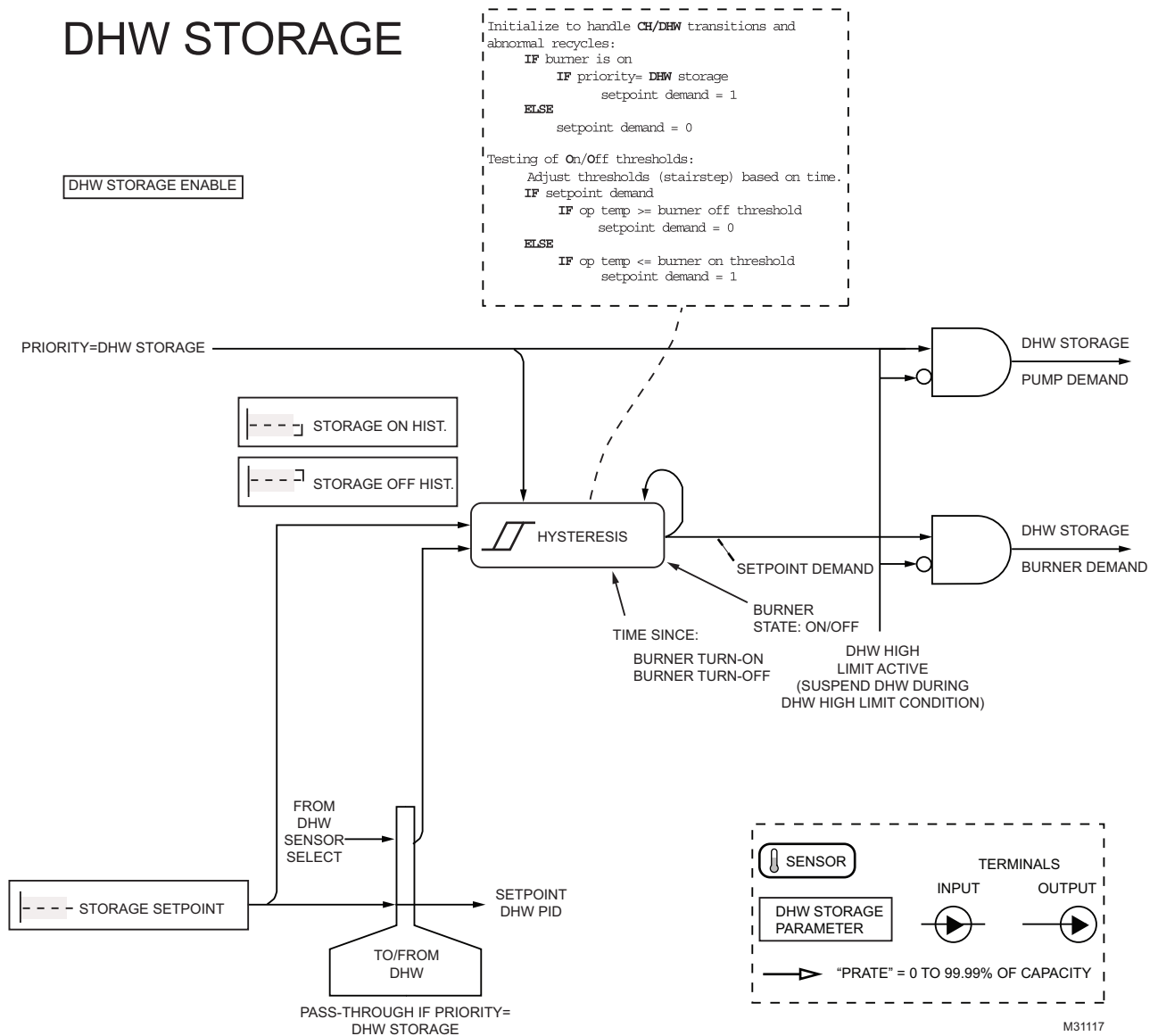
Fig. 16. DHW storage.
