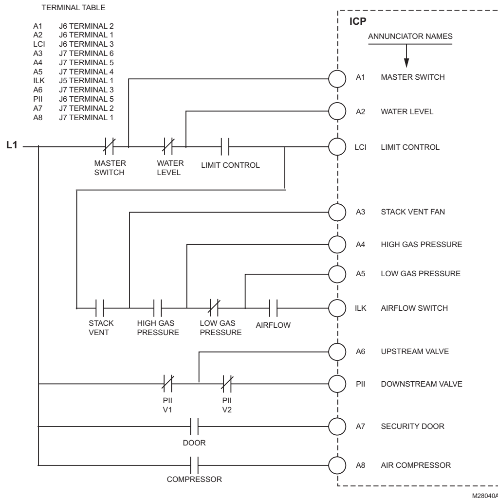
Fig. 26. Example of annunciator inputs and terminal names.
