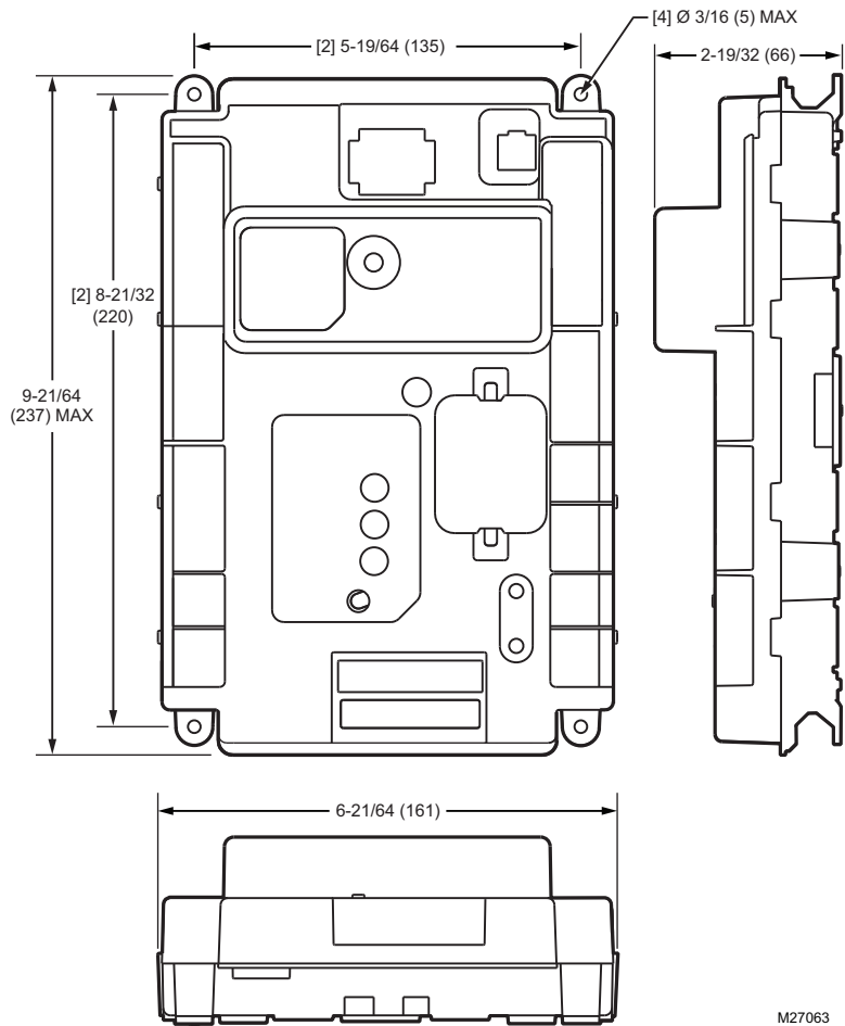
Fig. 2. R7910A/R7911 dimensions in in. (mm).
