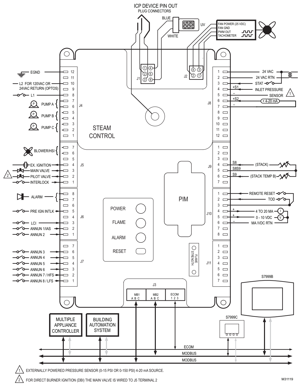
Fig. 4. R7911 device pin out.
