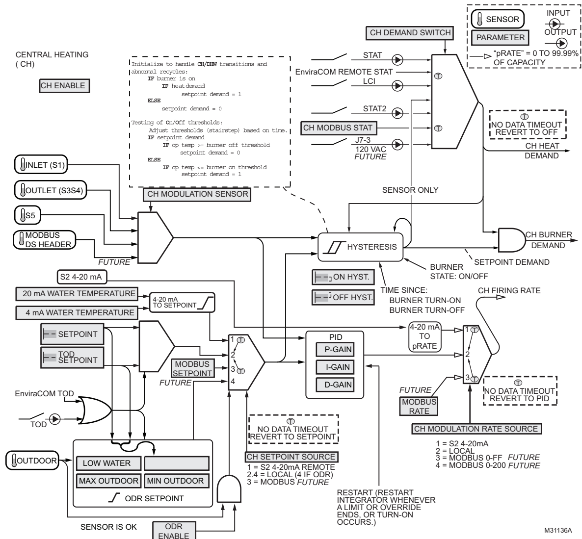
Fig. 8. Central heating hydronic diagram.
