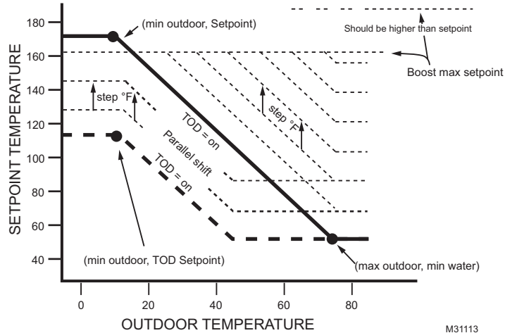
Fig. 9. Outdoor reset with TOD and boost.
