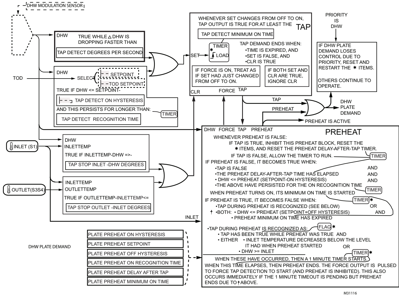
Fig. 15. Plate heat exchanger subsystem.
