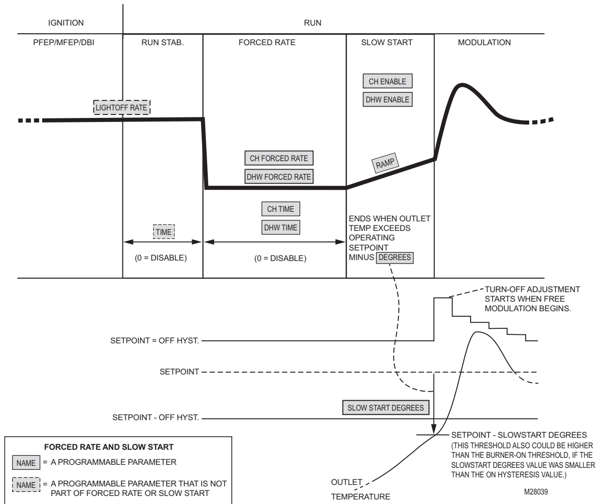
Fig. 20. Slow Start and Forced Rate limits.
