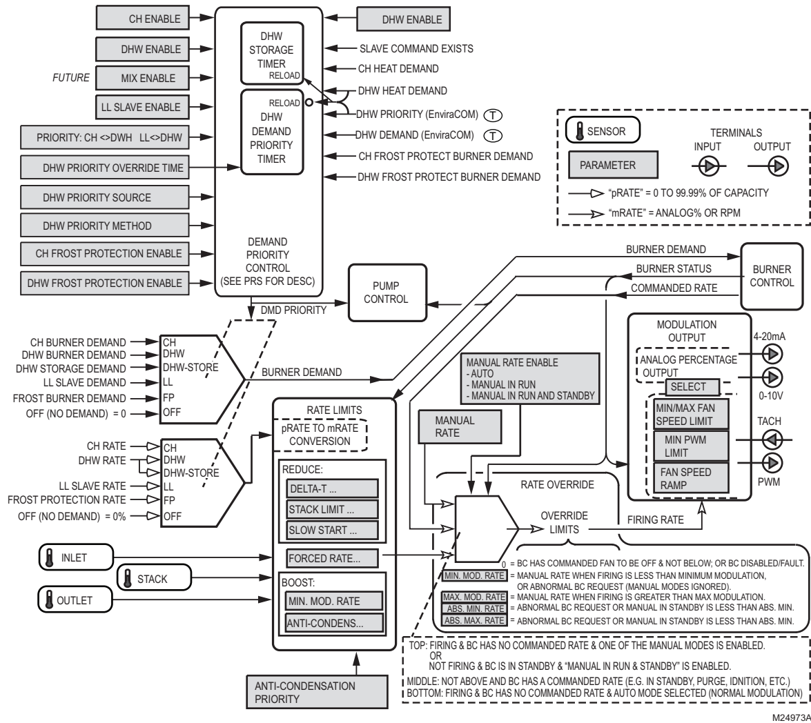
Fig. 5. Demand and rate selection diagram.
