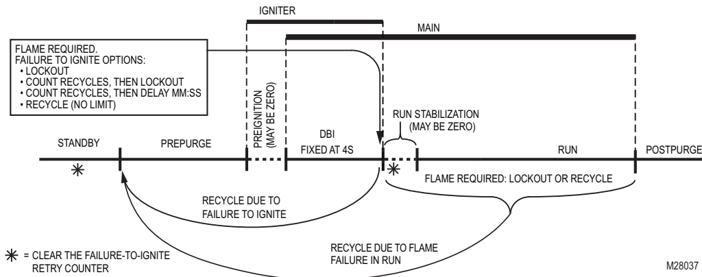
Fig. 25. Direct burner ignition
