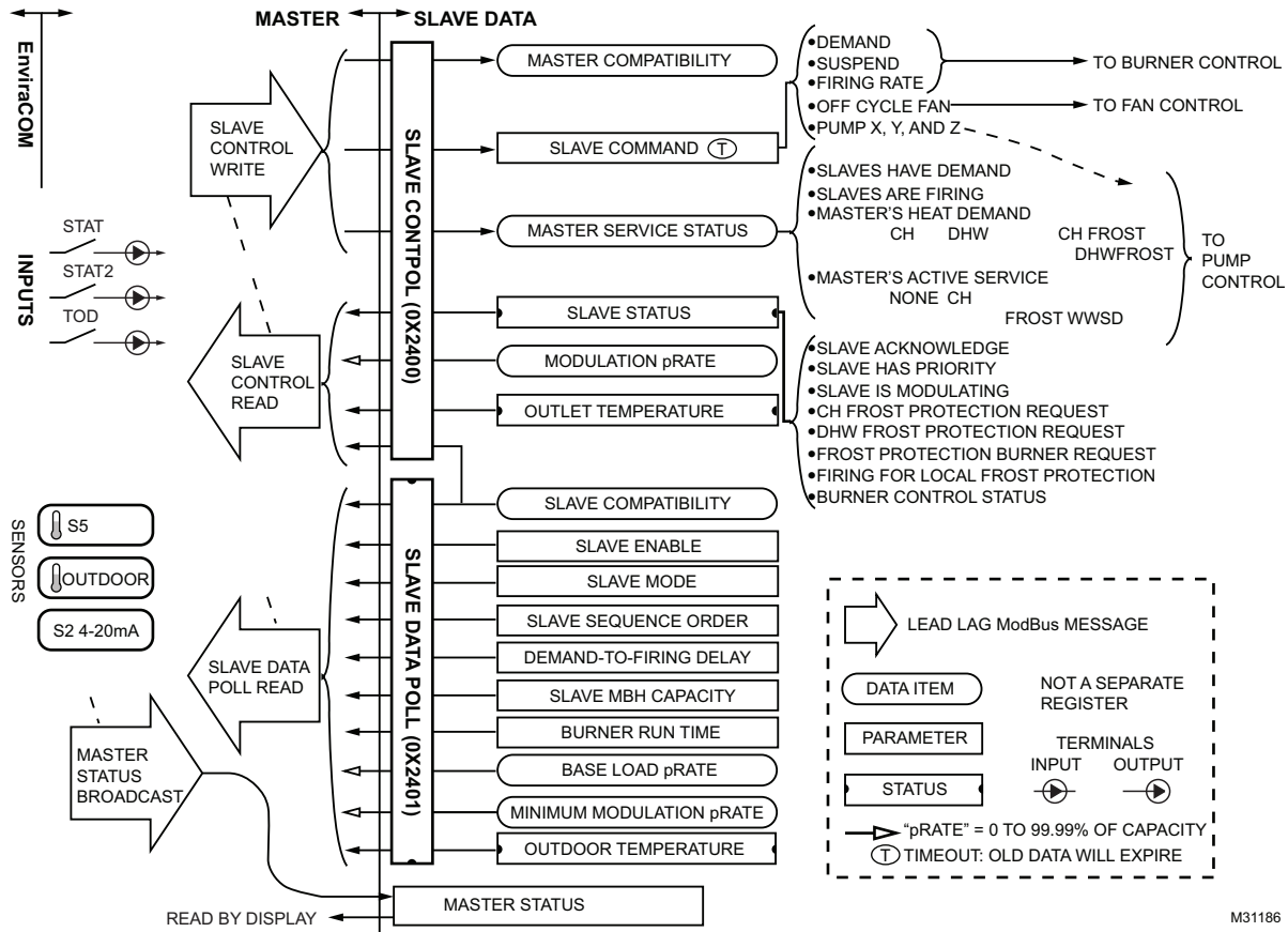
Fig. 29. Master/Slave data transmission.
