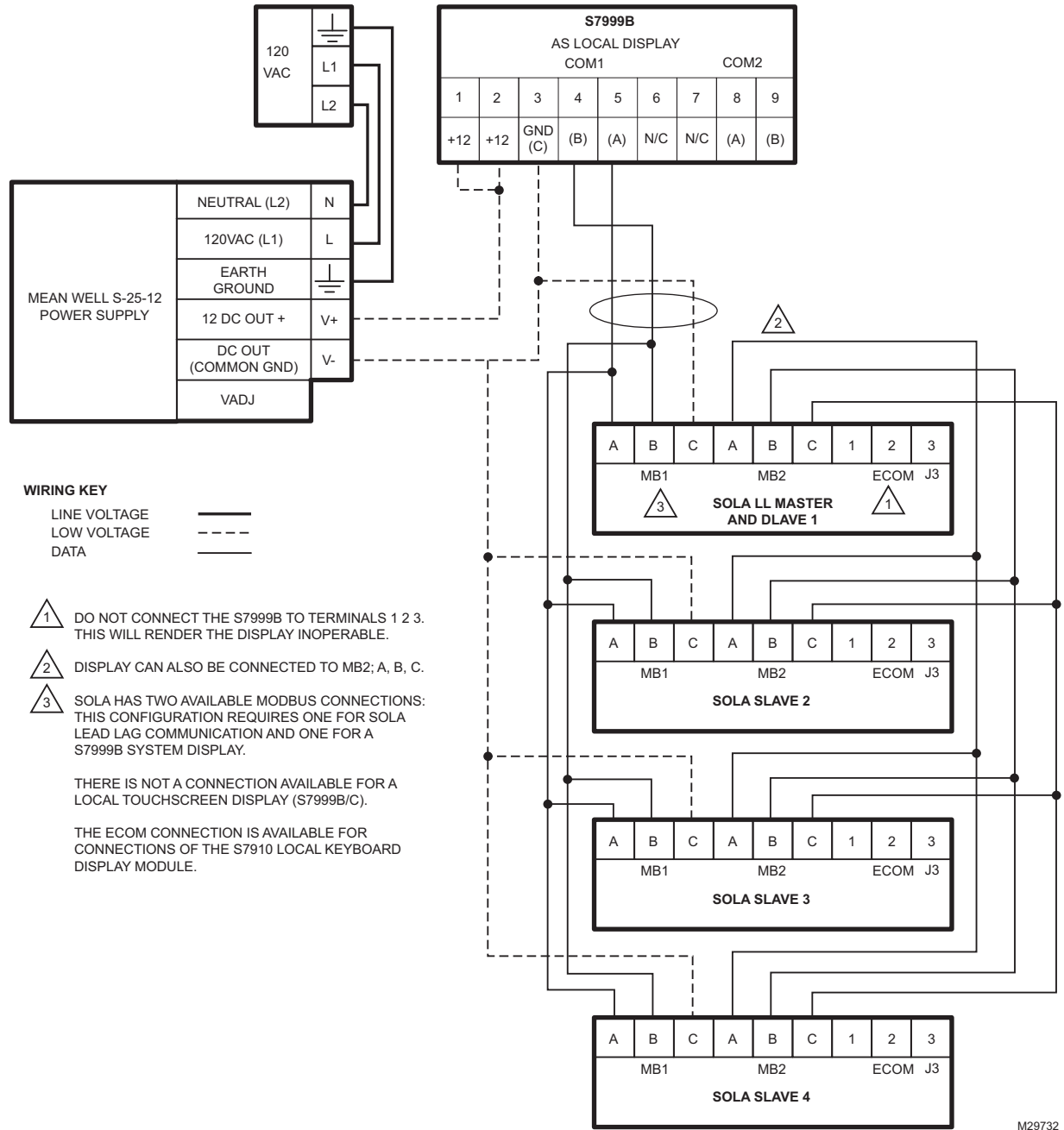
Fig. 28. S7999B system and lead lag wiring diagram.
