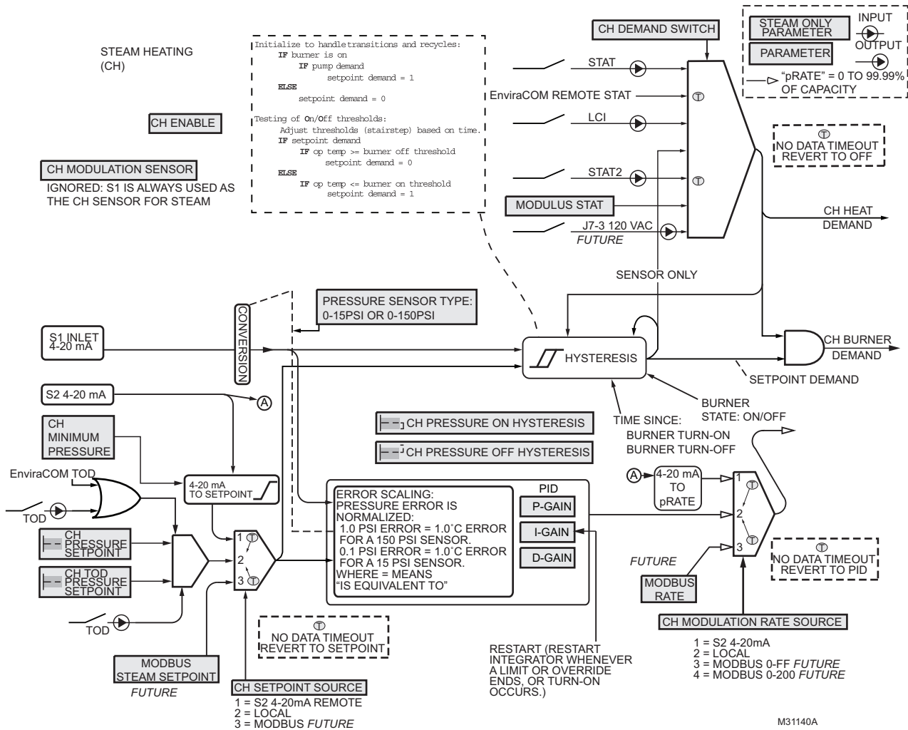
Fig. 11. Central heating steam diagram.
