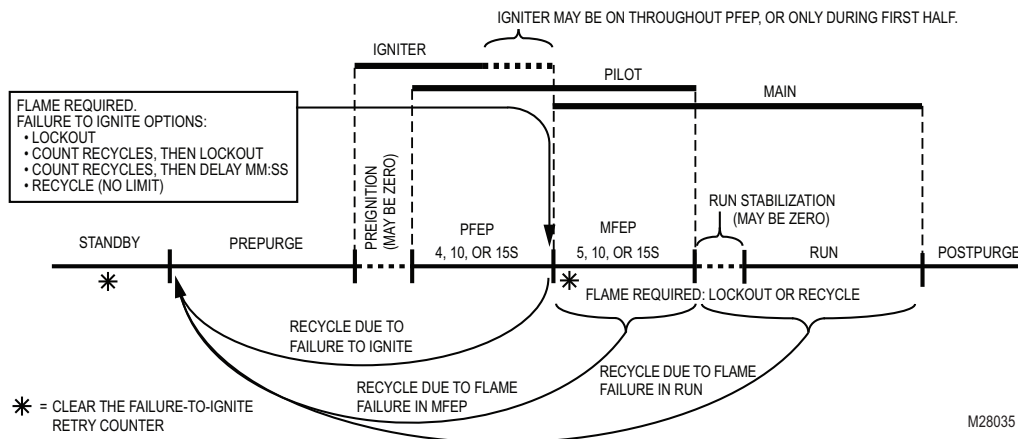
Fig. 23. Interrupted pilot.
