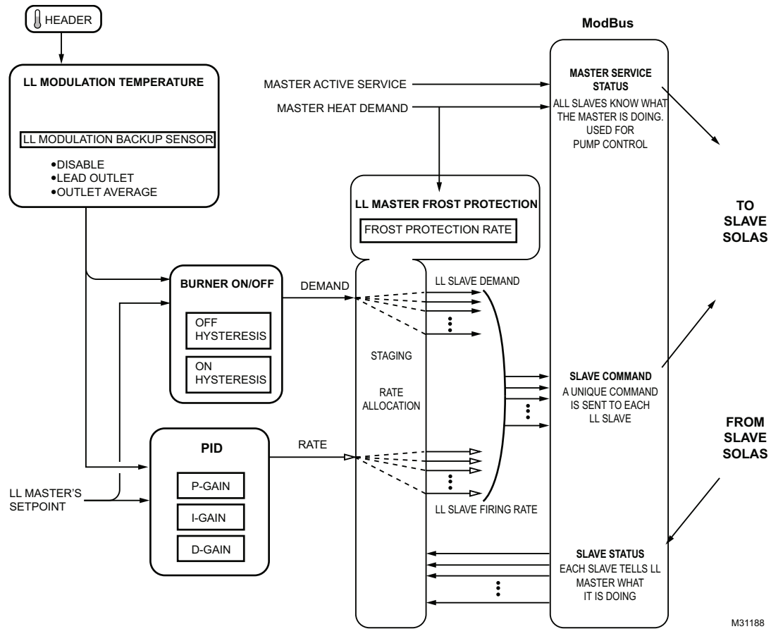
Fig. 31. Modulation.
