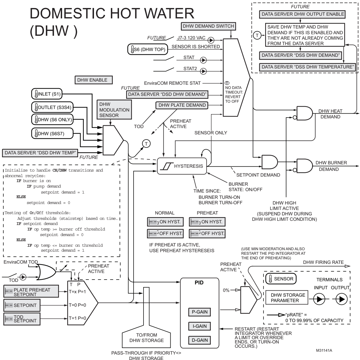
Fig. 14. Domestic hot water function.
