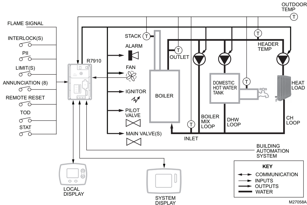
Fig. 1. General R7910 hydronic boiler schematic.
