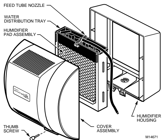
Fig. 4. Humidifier components.
