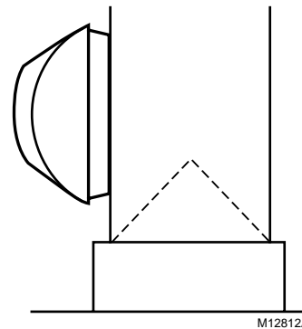
Fig. 3. HE365 Humidifier location in relation to air conditioning cooling coils.
