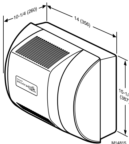
Fig. 1. HE365A,B dimensions in in. (mm).
