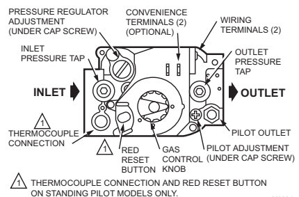
Fig. 1. Top view of VR8200 combination gas control.
