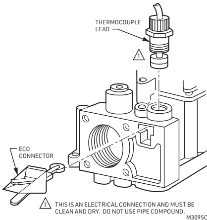
Fig. 1. Install ECO connector into gas control at thermocouple terminal location.
