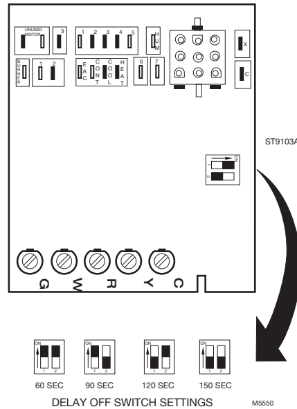
Fig. 3. Setting delay off switches.
