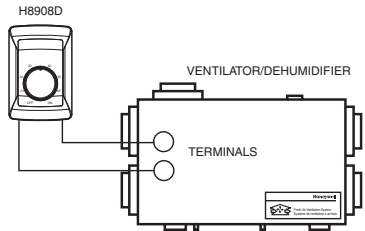
Fig. 18. Typical wiring diagram for HR150, HR200, ER150 and ER200 Ventilator or DH90 Dehumidifier applications.
