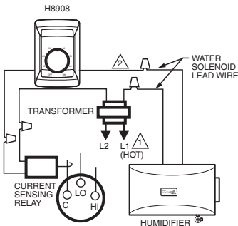
Fig. 14. Typical wiring diagram of current sensing relay with humidifier.
