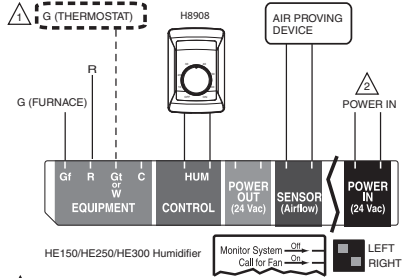
Fig. 16. Wiring H8908 with steam humidifiers.
