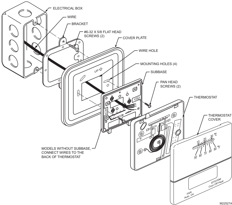
Fig. 3. Mount bracket, cover plate, subbase and thermostat to a vertical 2 in. X 4 in. electrical box.
