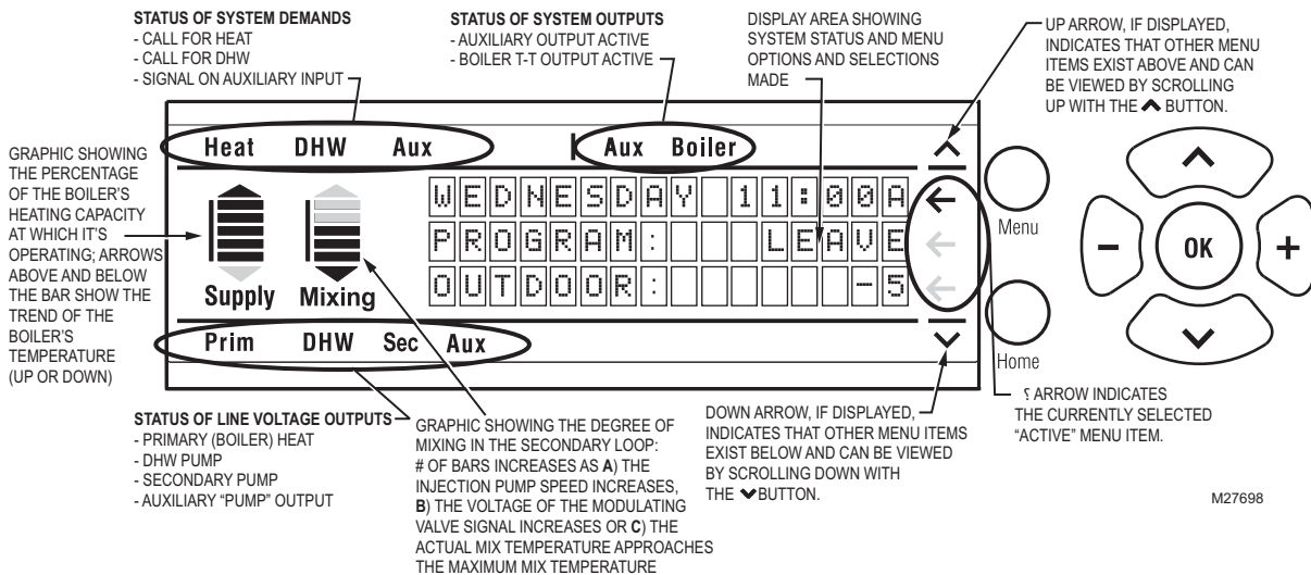
Fig. 1. LCD display and keypad layout.
