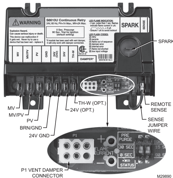
Fig. 1. Typical wiring connections.
