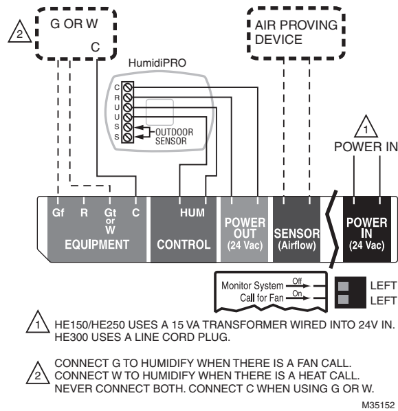
Fig. 1. Wiring HumidiPRO (H6062) to humidify only with a call for Heat or Fan.
