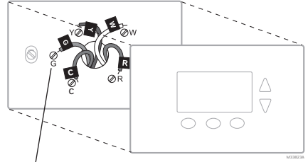
Terminal designation
