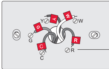
Terminal designation
